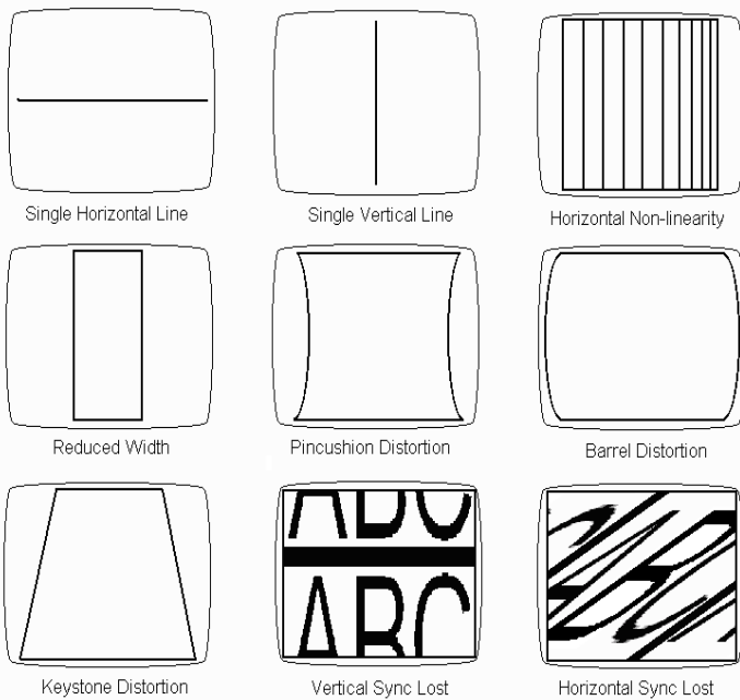
Symptoms of Some Common Deflection Problems
